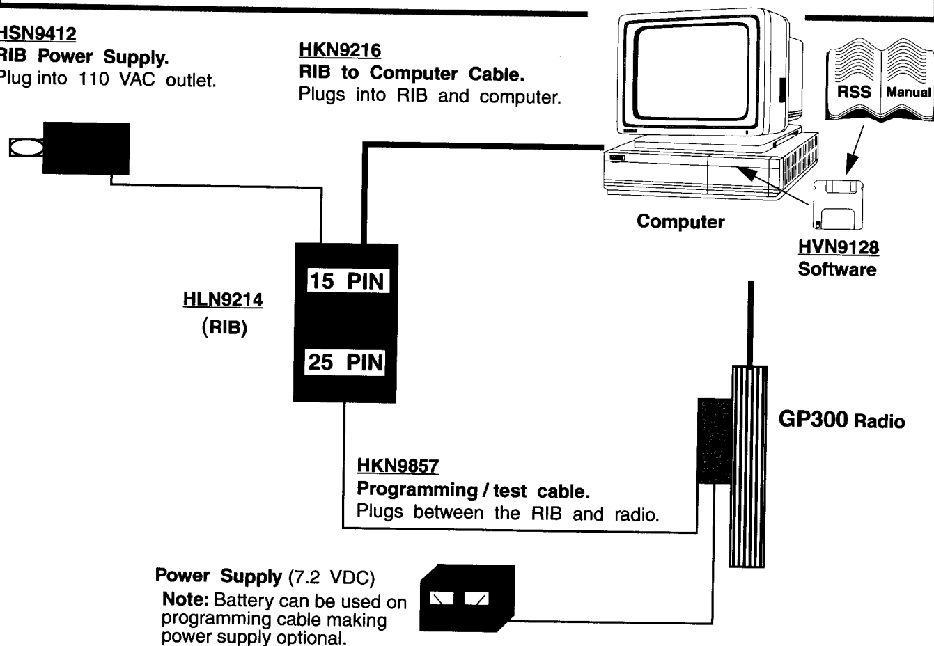
Figure 2. Equipment Setup
