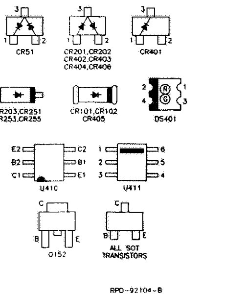
Schematic Diagram for HLE8055B and HLE8057B UHF Main Boards, 490-520 MHz (sheet 1 of 2)
